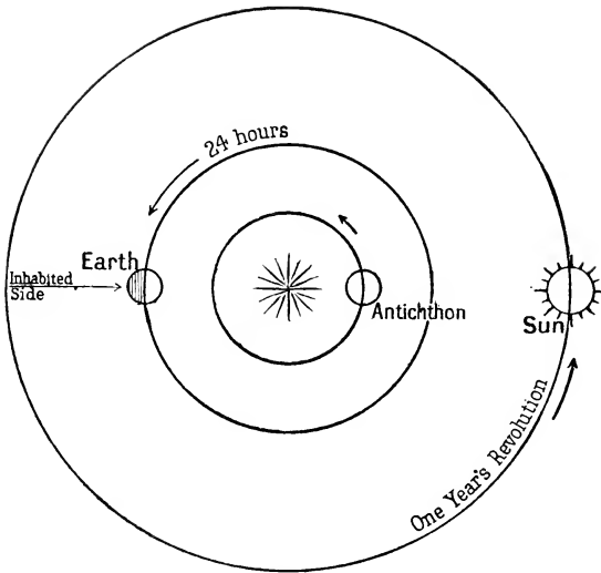
Fig. 16. The System of Philolaus : night on earth.
